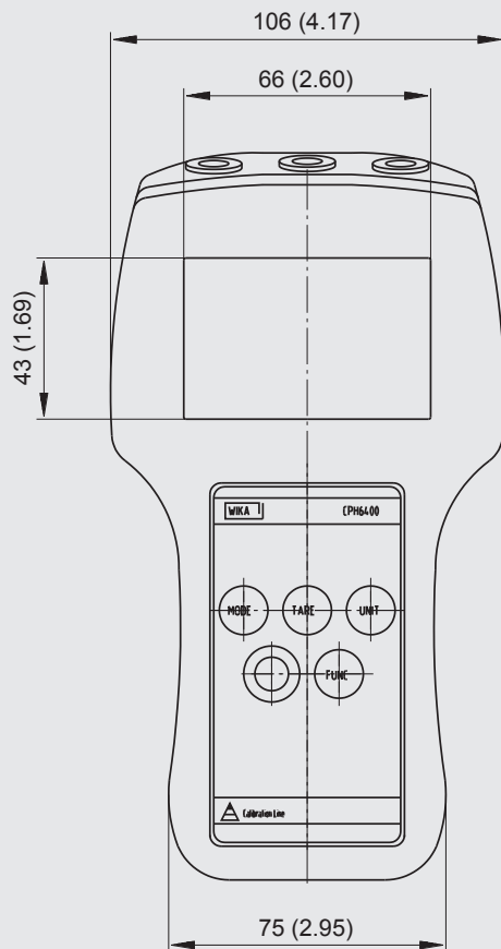
Digital indicator CPH6400
